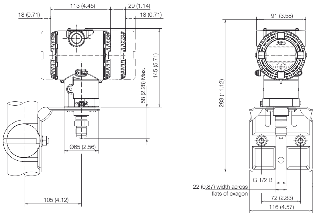
Transmitter with barrel housing - DIN-EN837-1 G 1/2 B connection
